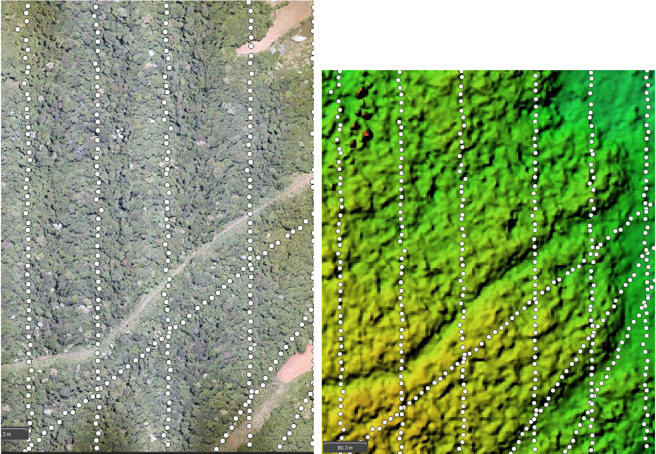
Figure 2. The capture of an orthomosaic and and de DEM in the processing workflow of X3 camera. Lowest quality was applied.
